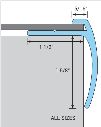
Stair Nose
